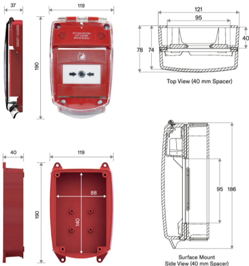
Dimensions (mm)
